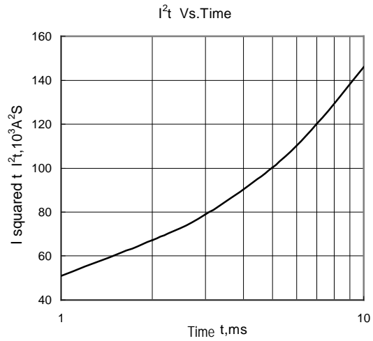
Fig.8 I^2t Vs.Time
