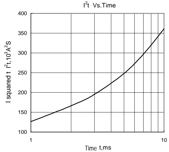
Fig.8 I^2t Vs.Time
