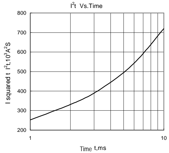
Fig.8 I^2t Vs.Time
