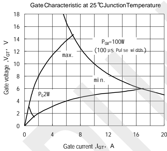
Fig.9 Gate Power Graph
