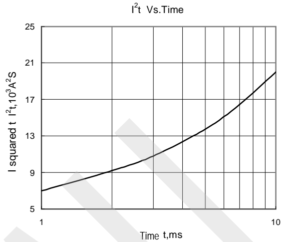
Fig.8 I^2t Vs.Time
